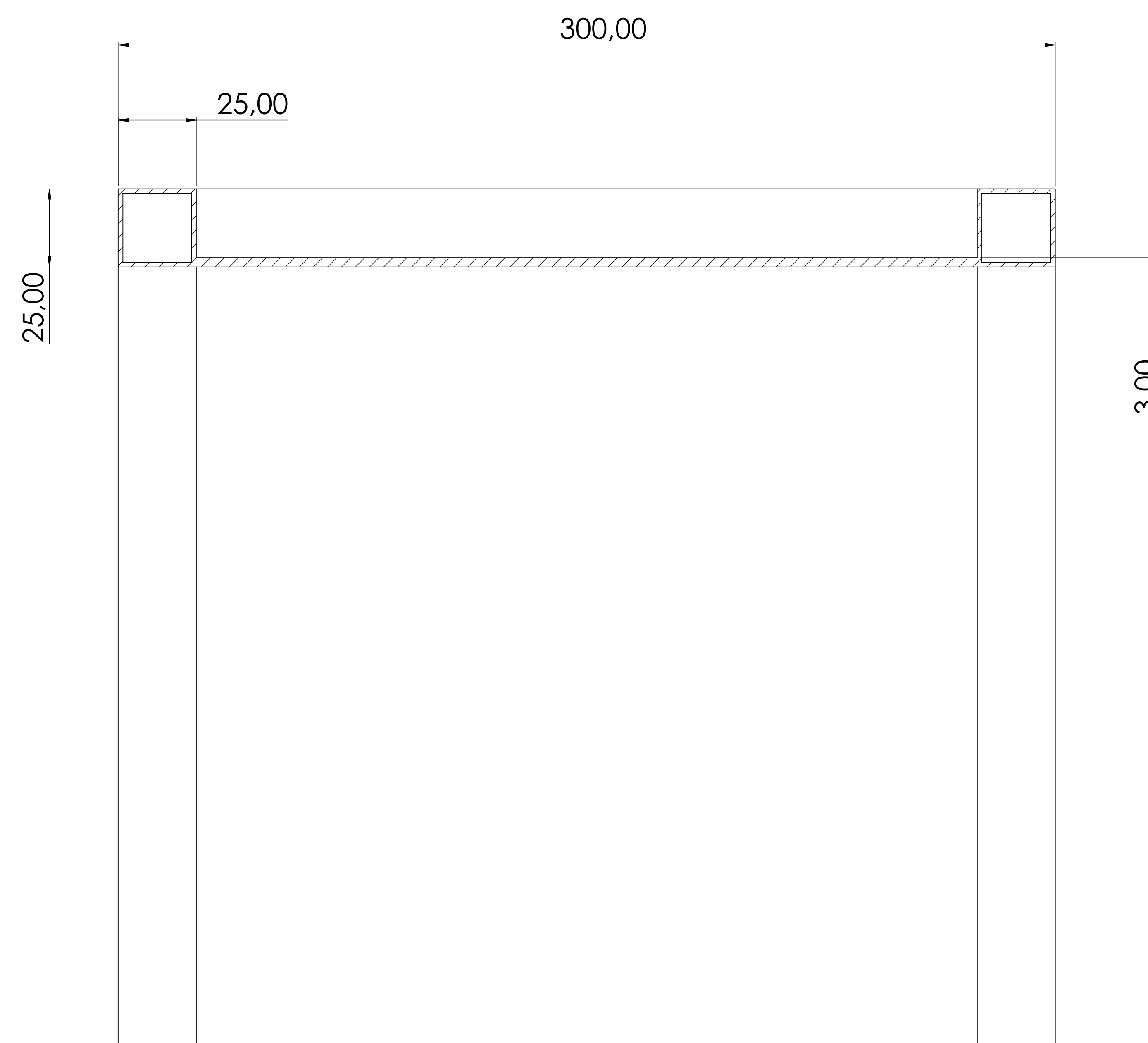
SECTION H-H
